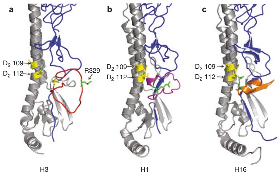
Fig. 1.3 Cleavage site structures showing a single monomer of the HA0 trimer for H3 subtype (a), H1 subtype (b), and H16 subtype (c). (a) The cleavage domain of H3 (red) forms a loop structure with R329 (green) oriented out into solution. Shown in yellow are residues that line the electronegative cavity, residues HA 2 D109, HA 2 D112 (subscript denotes the HA 2 subunit in the figure), and HA 1 His 17 (between D 2 112 and R329). (b) The cleavage domain of H1 (magenta) packs more closely against the trimer, but R329 (green) remains oriented out into solution. HA 2 D109, HA 2 D112, and HA 2 H111 are shown in yellow, though H111 is on the opposite face of the long helix and largely hidden in the depicted orientation. (c) The cleavage domain of H16 (orange) contains a small helical domain that orients the side chain of R329 (green) into the electronegative cavity, where it forms a salt bridge with HA 2 D112 (again, ionizable residues shown in yellow). In all panels, residues that will constitute the HA 1 and HA 2 subunits following cleavage are shown in blue and gray, respectively
